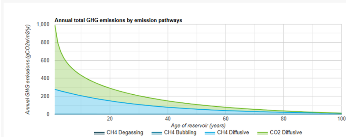
GHG Emissions by emission pathways
